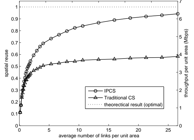
Fig. 5. Spatial reuse and network throughput under IPCS and the conventional CS mechanisms
