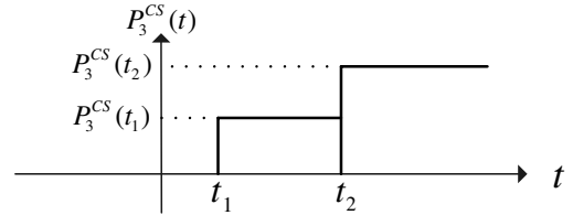
Fig. 4. The power sensed by transmitter T'_3 as a function of time
