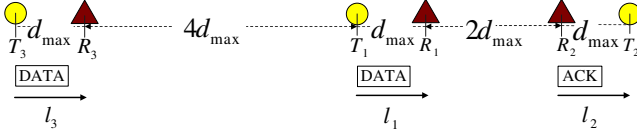
Fig. 1. Setting the carrier-sensing range as Safe-CSR pairwise is insufficient to prevent hidden-node collisions under the cumulative interference model
