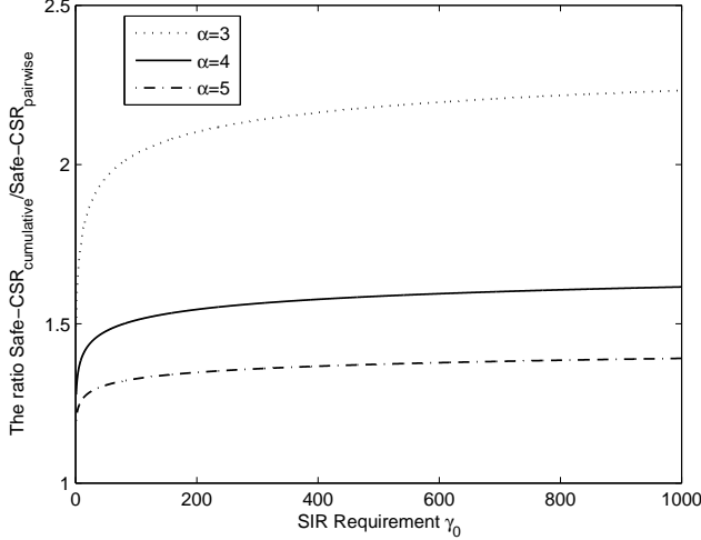
Fig. 2. The ratio of Safe-CSR_{cumulative} to Safe-CSR_{pairwise}
