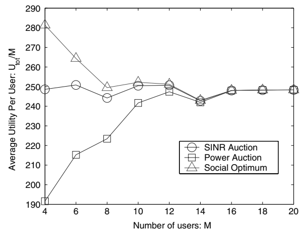
Figure 3. Utility comparisons in the large system limit of users with logarithmic utilities and co-located receivers: (P/n_0, B) = (10^4 M, 10^2 M) .
